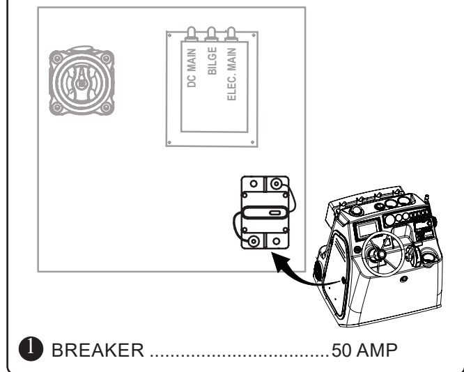
Trolling Motor Breaker Fig. 4.4.1
