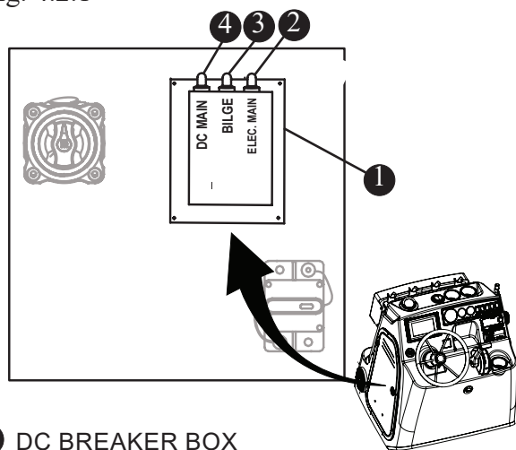
DC Main Breaker Box Fig. 4.2.1
