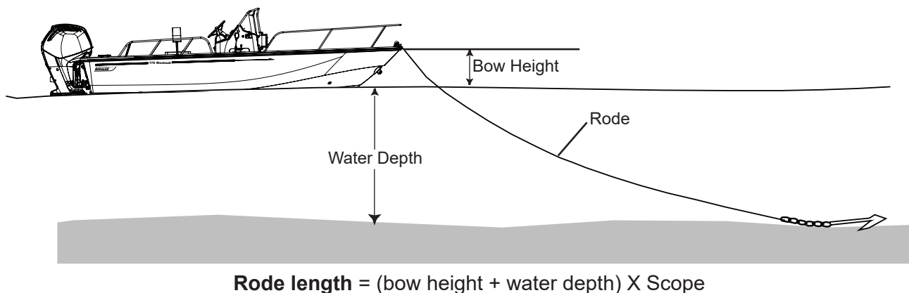
Proper Anchoring Fig. 3.11.1
