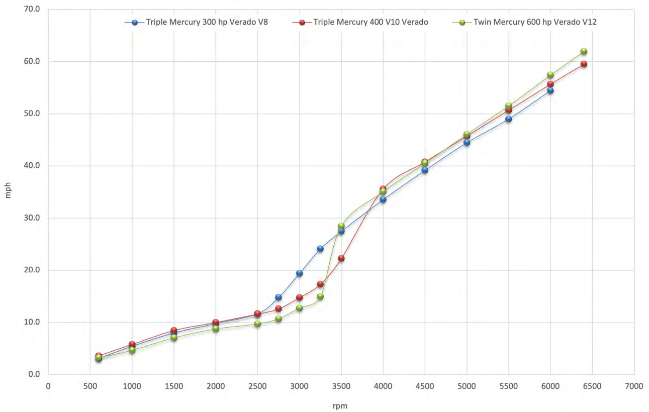
360 Outrage Engine Comparison Graph
