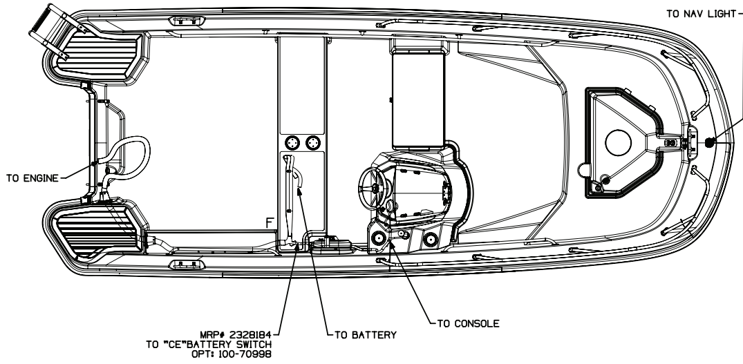
160 Super Sport Harness Diagram Fig.4.5.1
