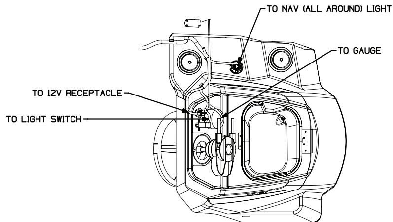
160 Super Sport Harness Diagram Fig.4.5.2
