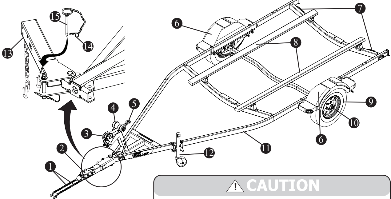
Single Axle Bunk Trailer Fig. 2.22.1
