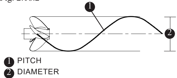
Propeller Pitch & Diameter Fig. 2.18.2
