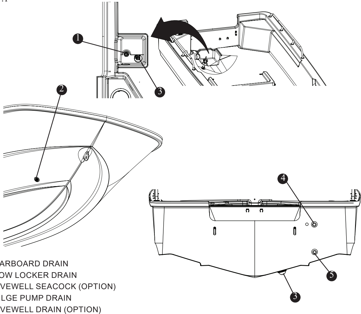
Through Hull Fittings Fig. 2.7.1
