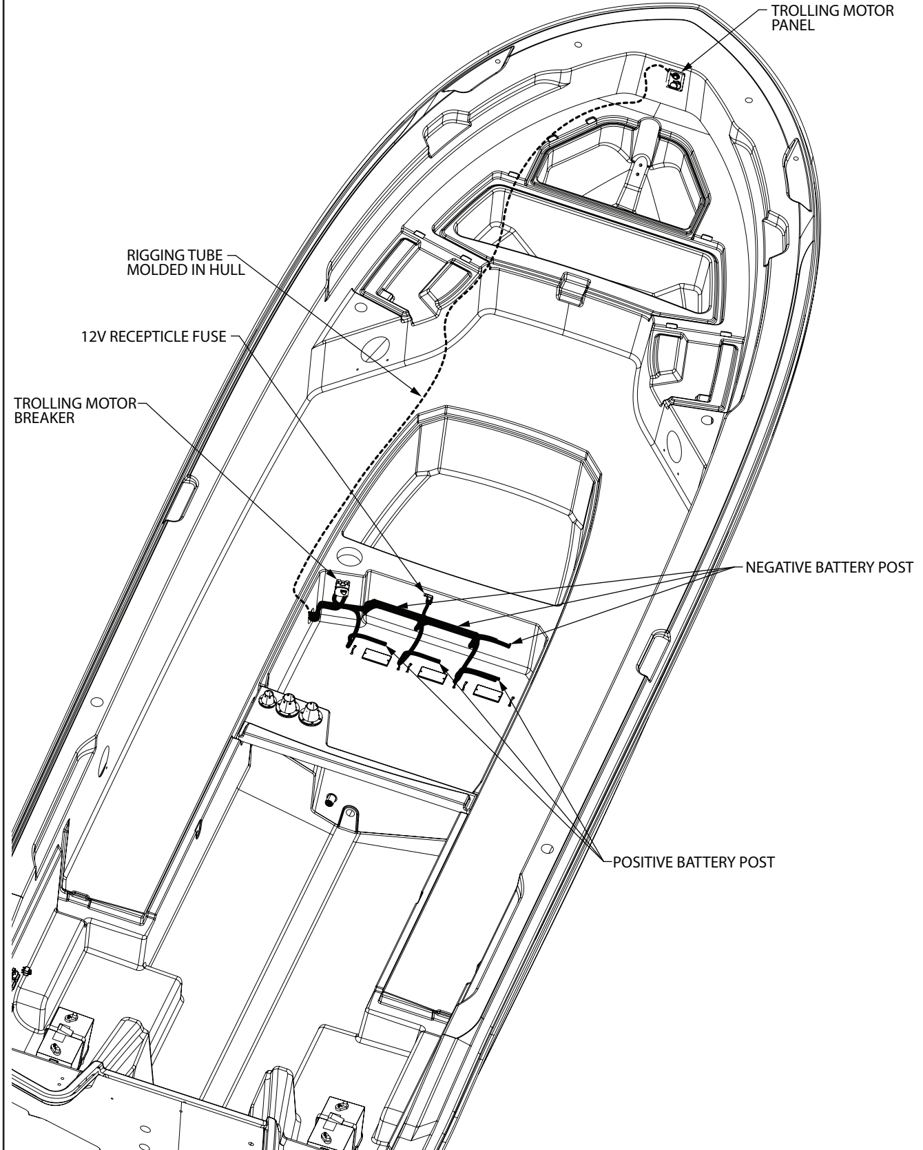
Trolling Motor Harness (Option) Figure 4.20.1
