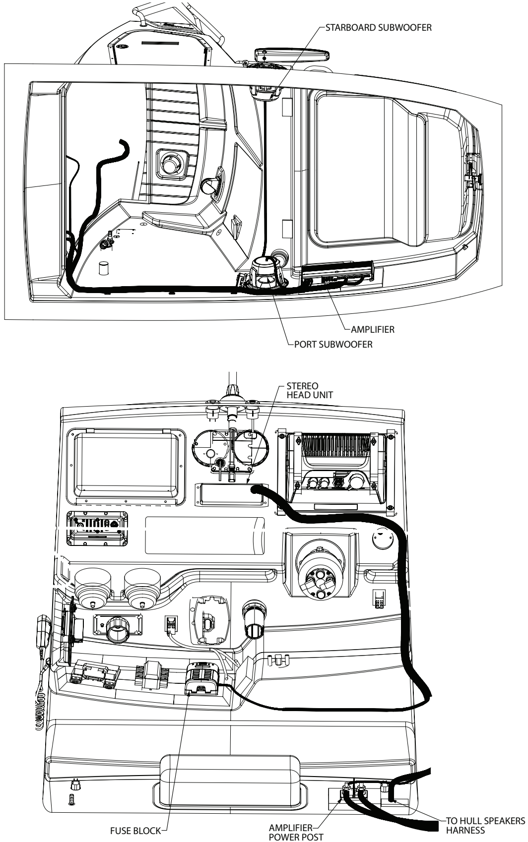
Stereo with Amplifier Harness (Option) Figure 4.19.1
