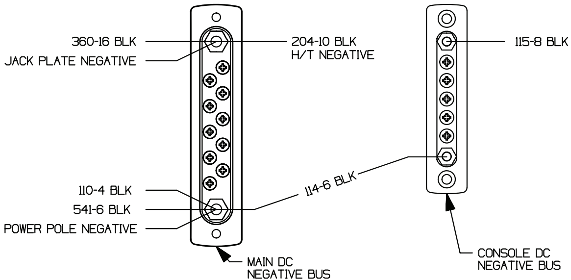
DC Negative Bus Figure 4.24.2
