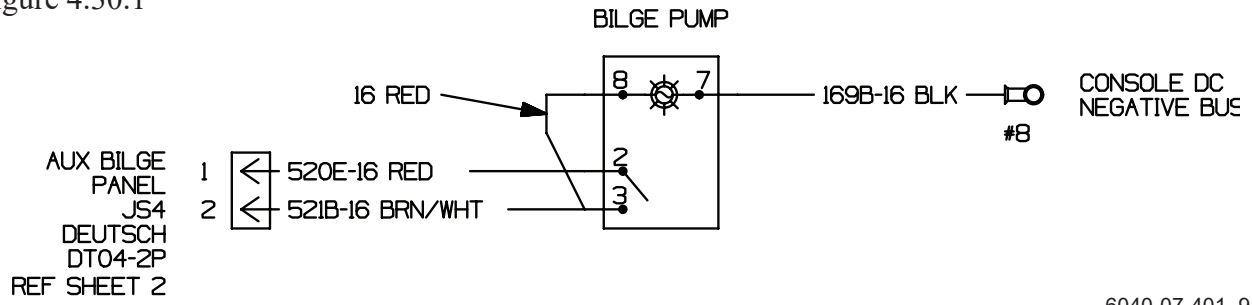
CE Auxiliary Bilge Pump (Option) Figure 4.30.1
