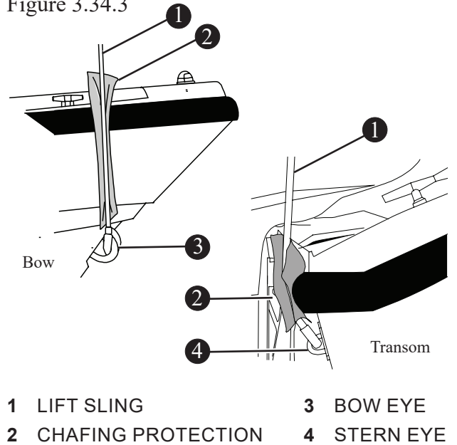
Short-term Lifting Figure 3.34.3
