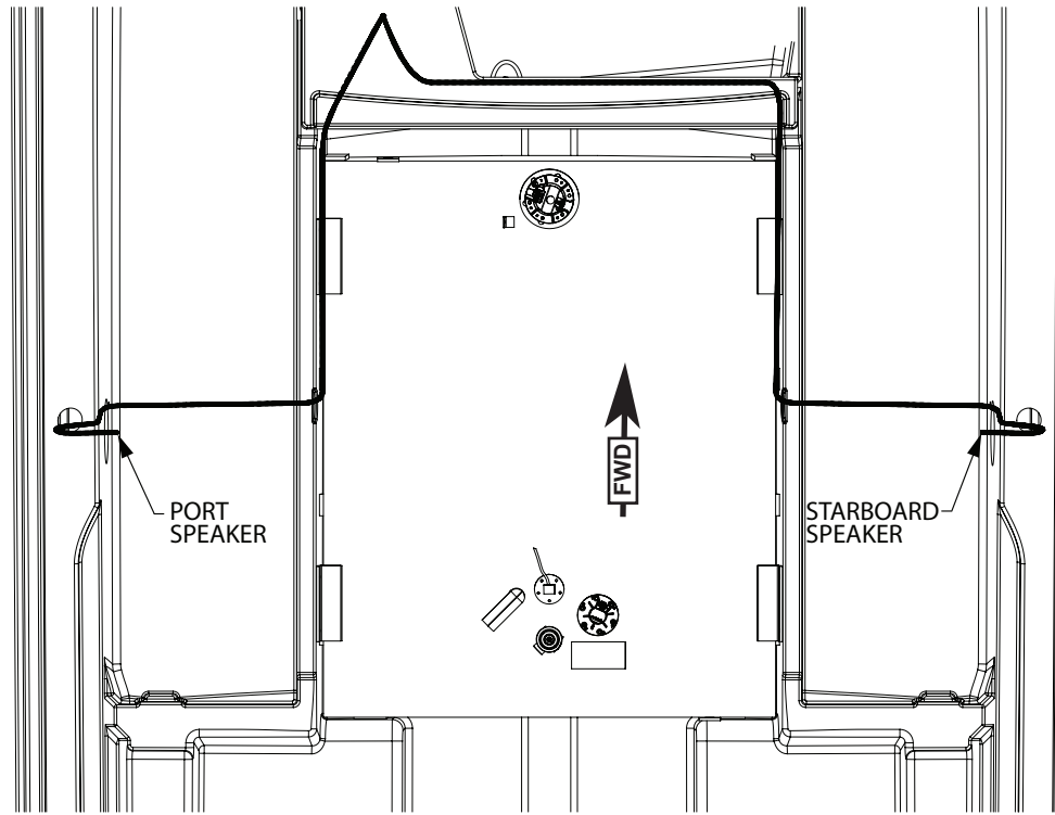
Stereo Speakers Harness (Option) (page 2 of 2) Figure 4.17.1
