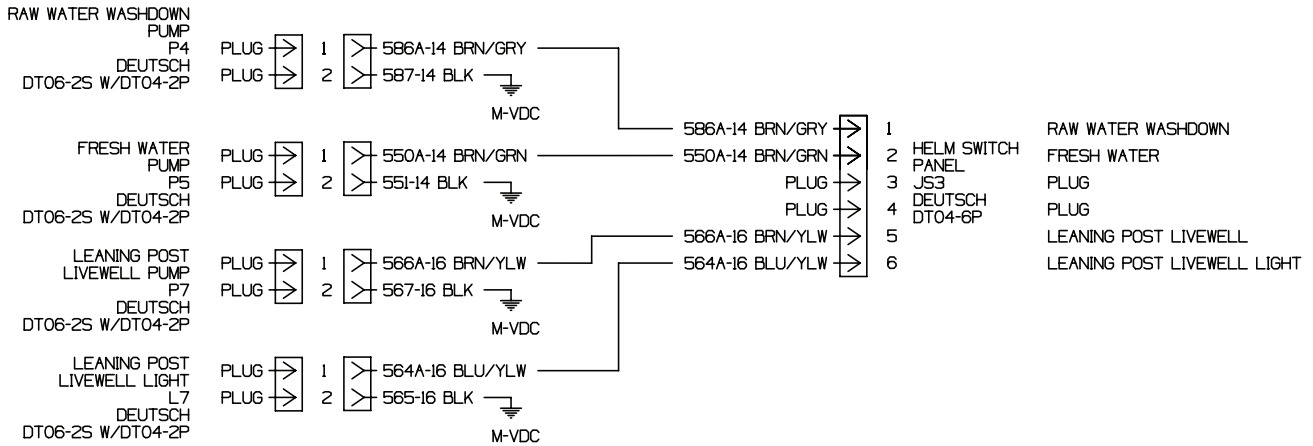
Water System (Option) Figure 4.30.2
