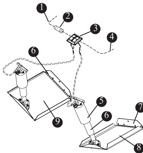
Electrically Powered Trim Tabs Fig. 2.22.1
