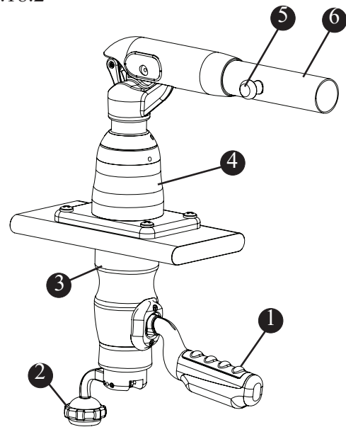
Radial Outriggers (Option) Fig. 3.18.2
