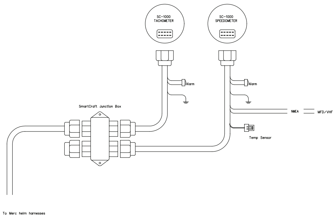
Instrument diagram (Single Engine)
