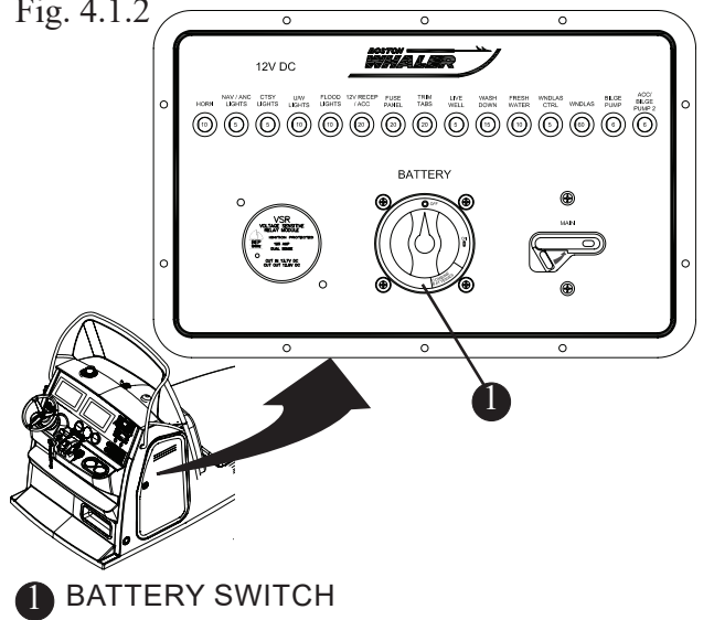
Battery Switch
