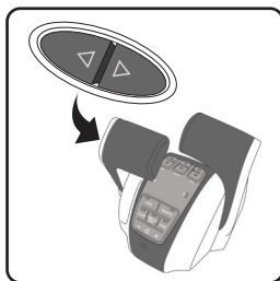
DTS Throttle Control (Dual Engine Option) Fig. 2.20.1
