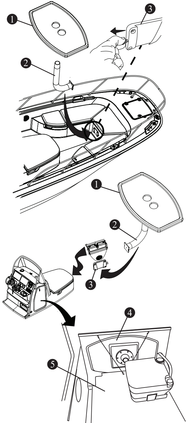
Bow Table (Option) Fig. 3.17.2
