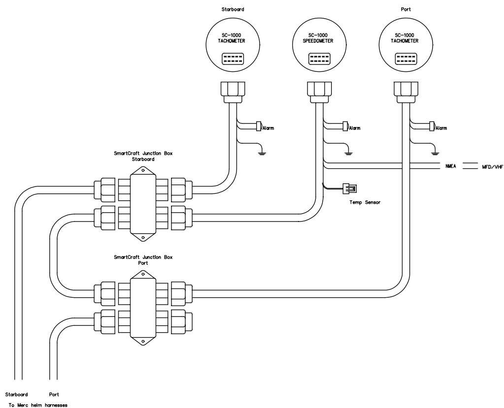
Instrument diagram (Dual Engine) (Option)
