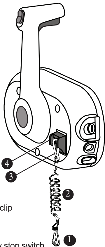
Engine Emergency Stop Switch Fig. 1.16.1
