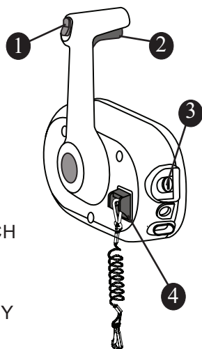
Throttle & Shift Control Fig. 2.10.1
