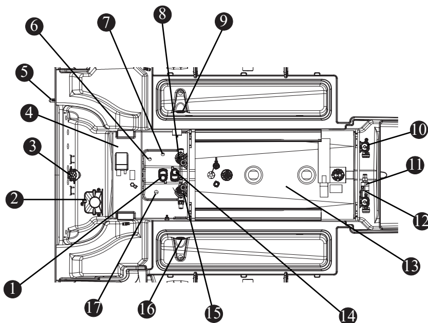
Bilge Layout
