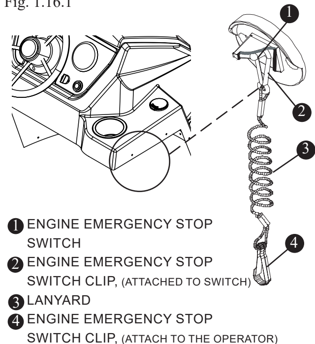
Engine Emergency Stop Switch Fig. 1.16.1
