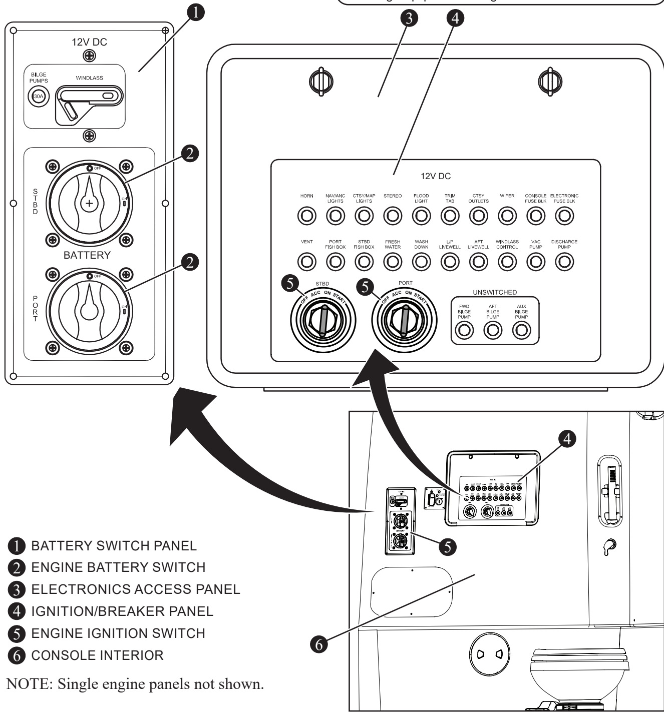
Ignition/Breaker Panel Figure 3.2.1
