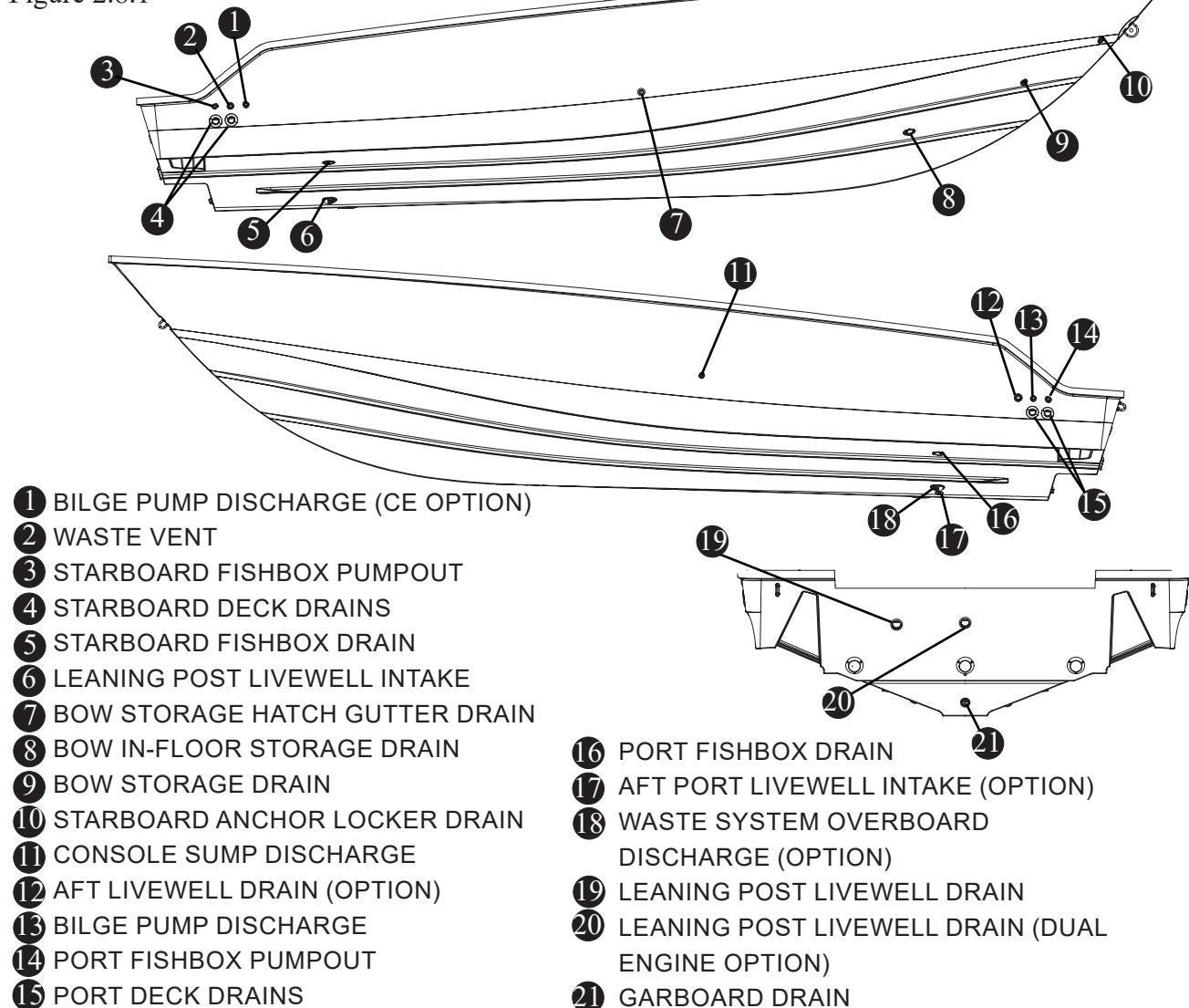
Through Hull Fittings Figure 2.8.1
