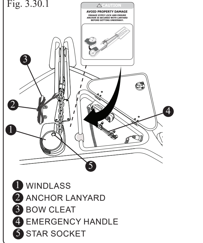
Windlass Manual/Emergency Operation Fig. 3.30.1
