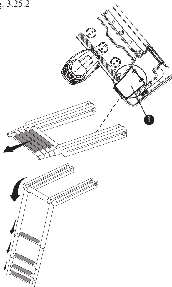
Retractable Swim Ladder Fig. 3.25.2
