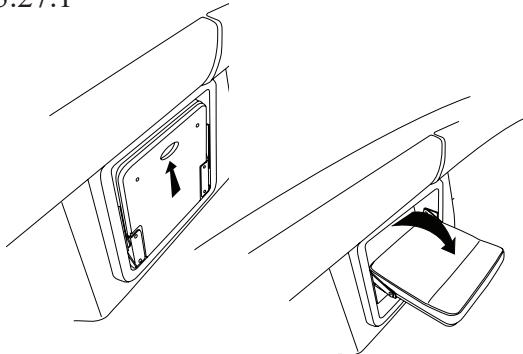
Foldaway Trolling Seat (Option) Fig. 3.27.1
