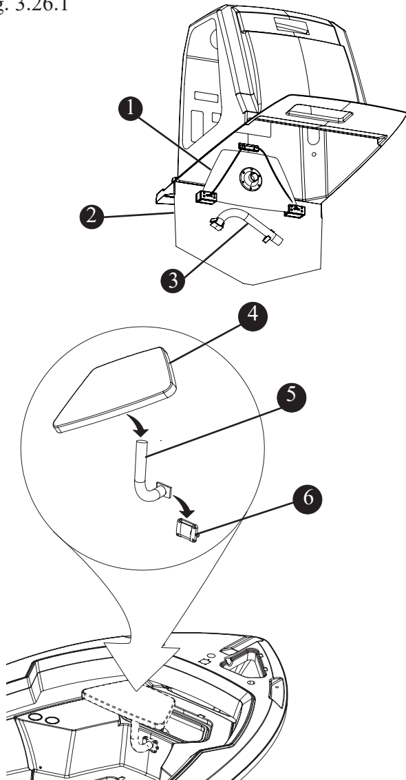
Bow Table (Option) Fig. 3.26.1
