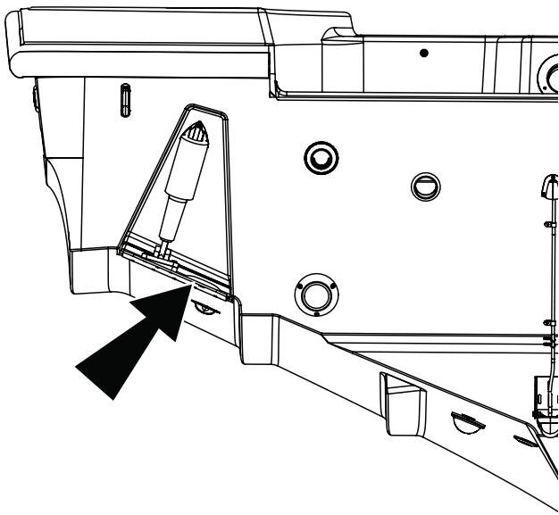
Trim Tabs Figure 3.5.1
