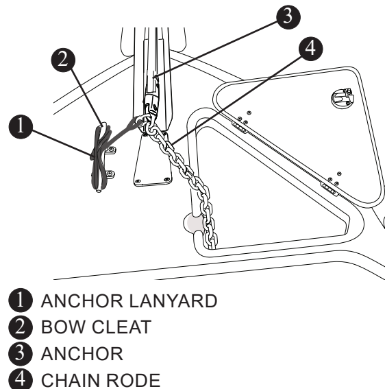
Manually Securing the Anchor Fig. 3.30.2
