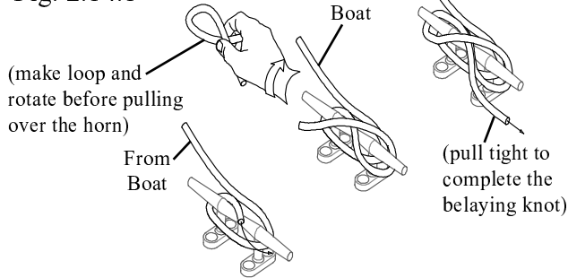
Belaying Knot Fig. 2.14.1
