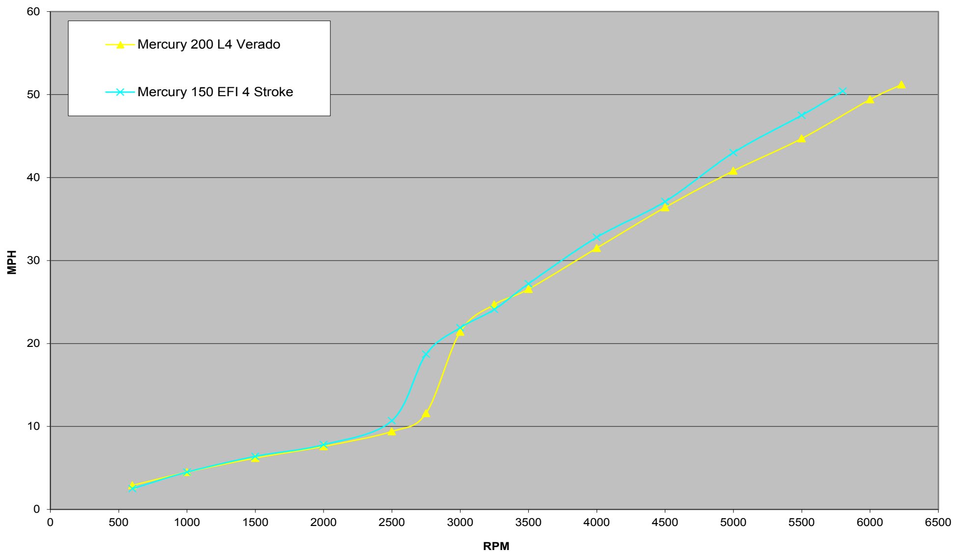
190 Outrage Engine Comparison Graph
